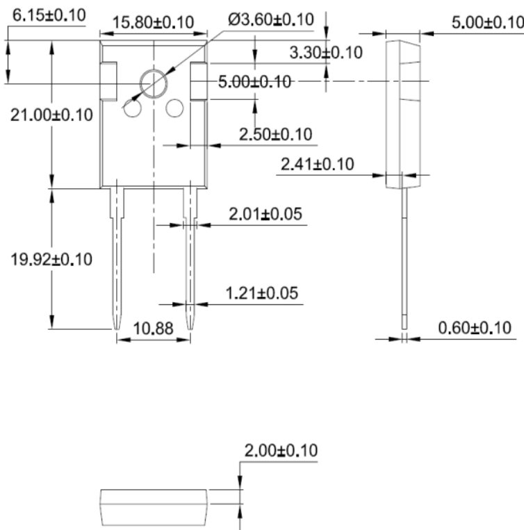
Figure 8. Package Outline
