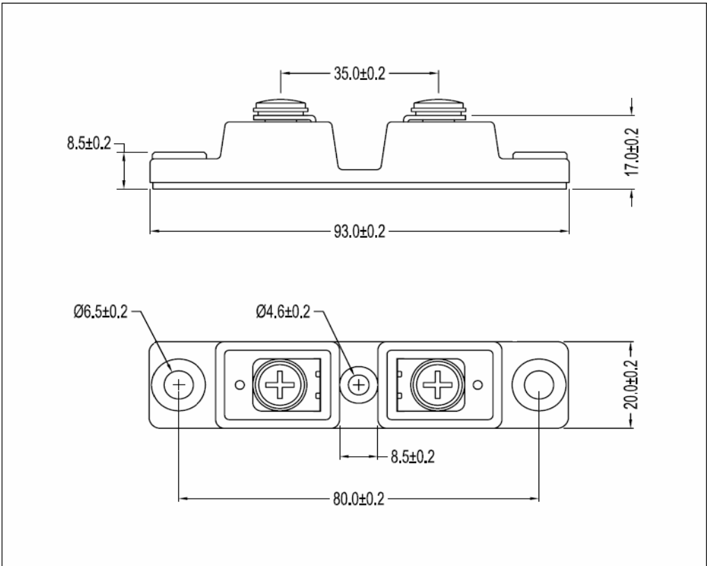
Dimensions (mm) Figure7. Package Outline
