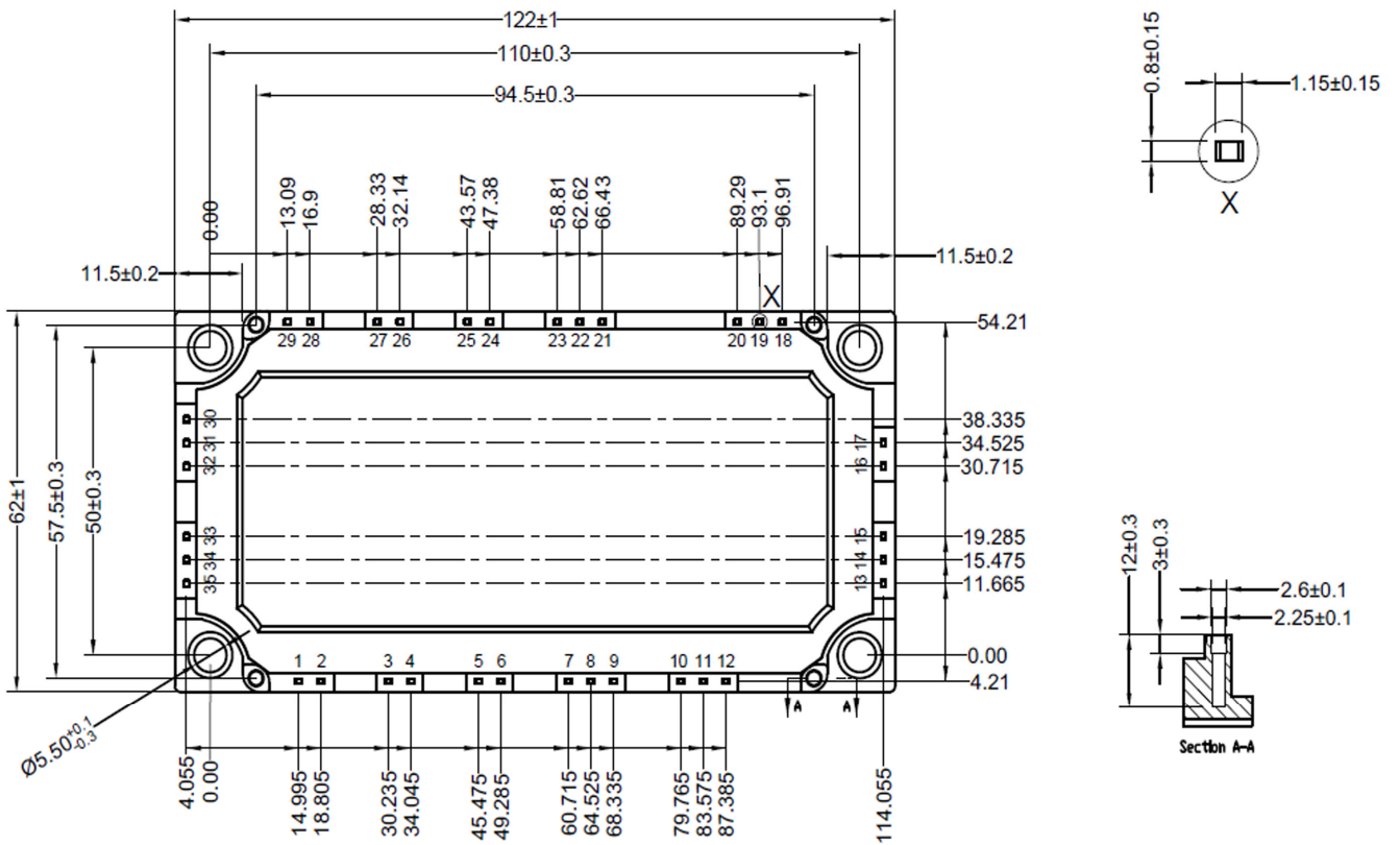
Dimensions in (mm) Figure 16. Package Outline
