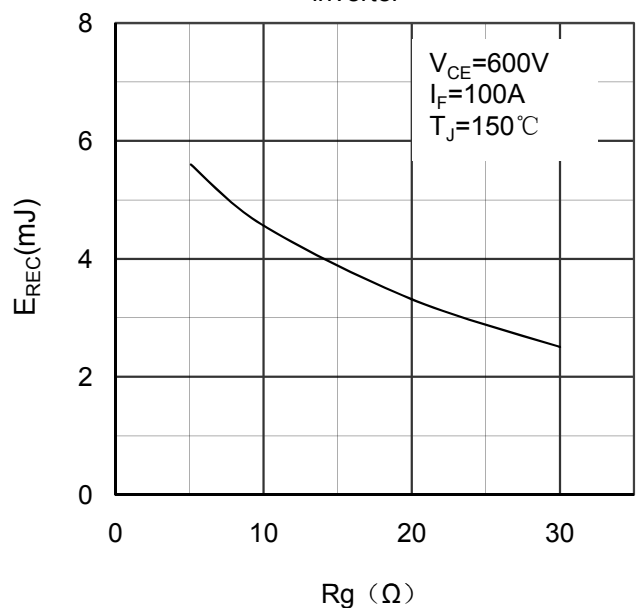
Figure 8. Switching Energy vs Gate Resistor Diode -inverter
