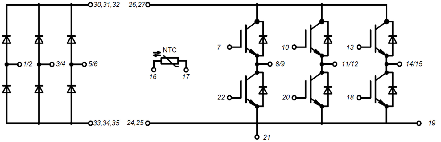
Figure 15. Circuit Diagram
