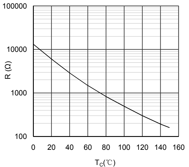
Figure 13. NTC Characteristics
