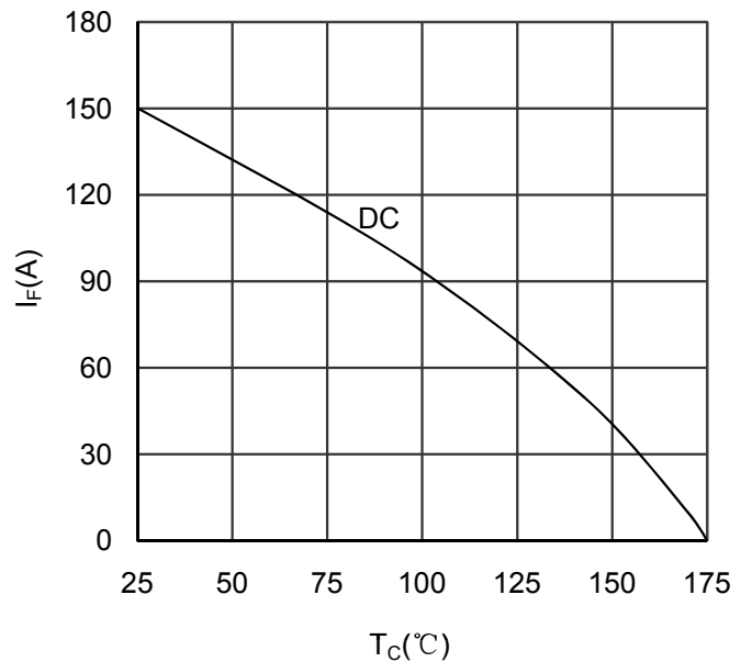
Figure 8. Forward current vs Case temperature Diode-inverter
