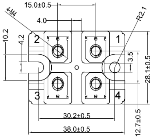
Dimensions in (mm) Figure 9. Package Outline
