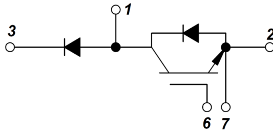
Figure 13. Circuit Diagram
