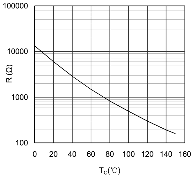
Figure 13. NTC Characteristics
