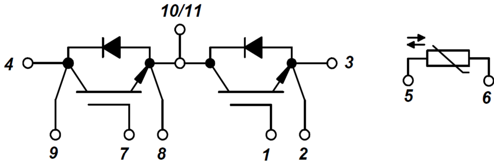
Figure 14. Circuit Diagram
