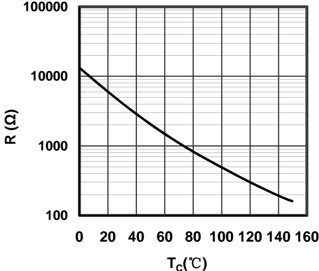
Figure 13. NTC Characteristics
