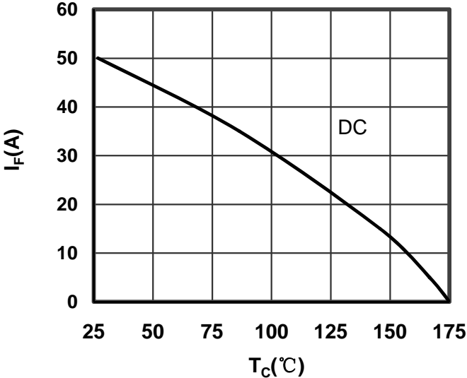
Figure 12. Forward current vs Case temperature Diode -inverter
