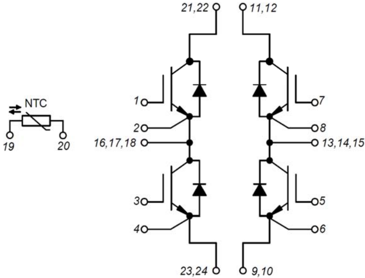
Figure 14. Circuit Diagram
