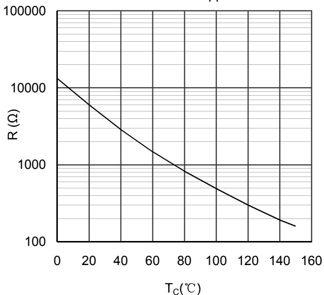
Figure 14. NTC Characteristics
